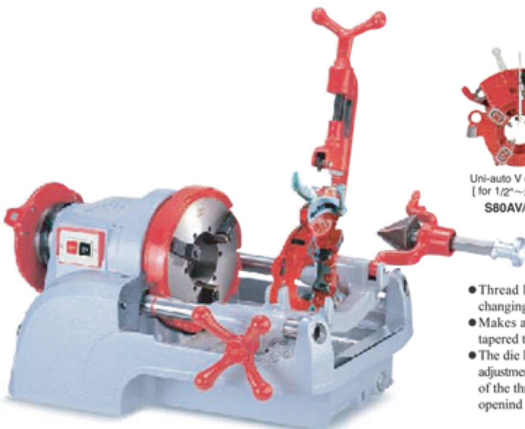
S80A with manual die head.
